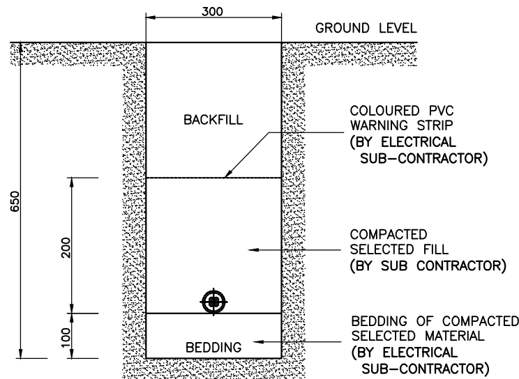
TELECOM TRENCH NTS
