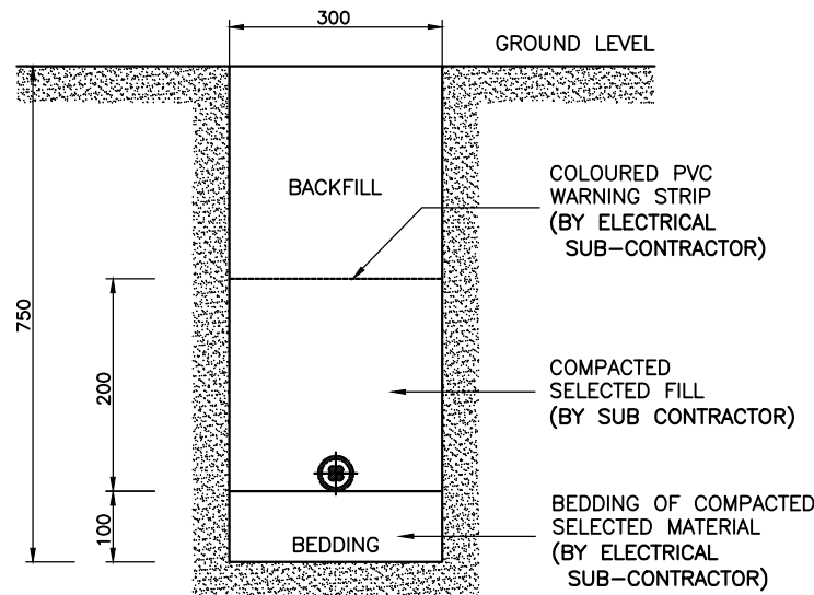
LOW VOLTAGE CABLES AND SLEEVES TRENCH NTS
